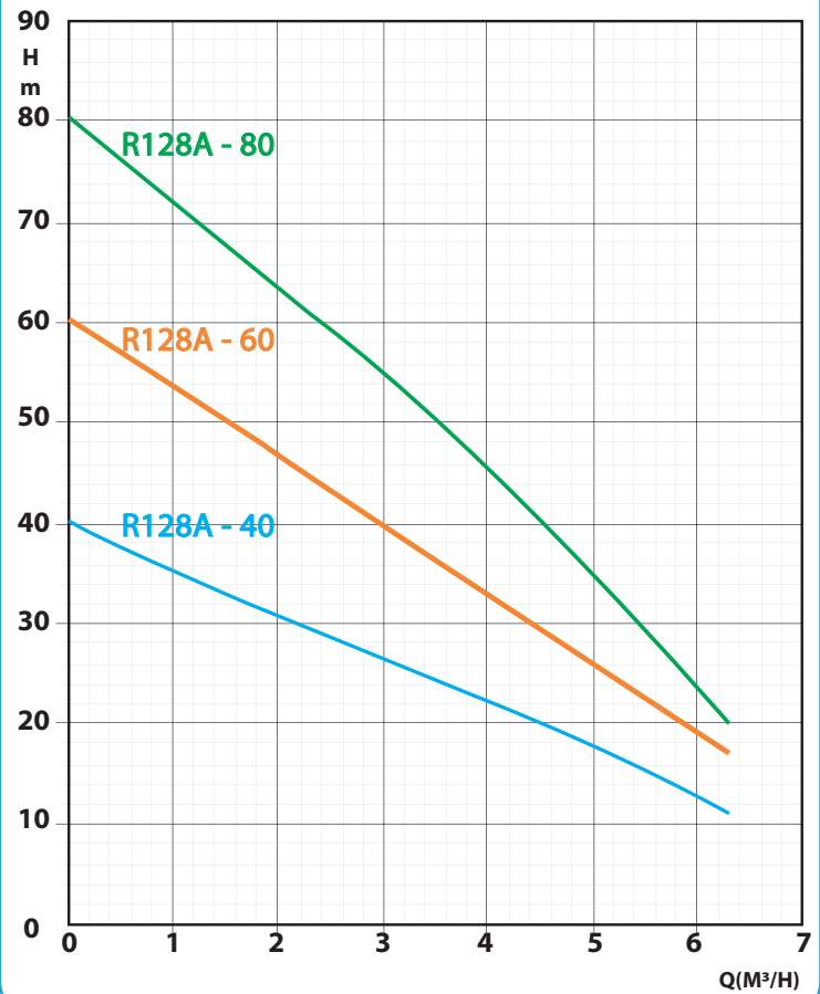
R128A Pump Performance Curve
