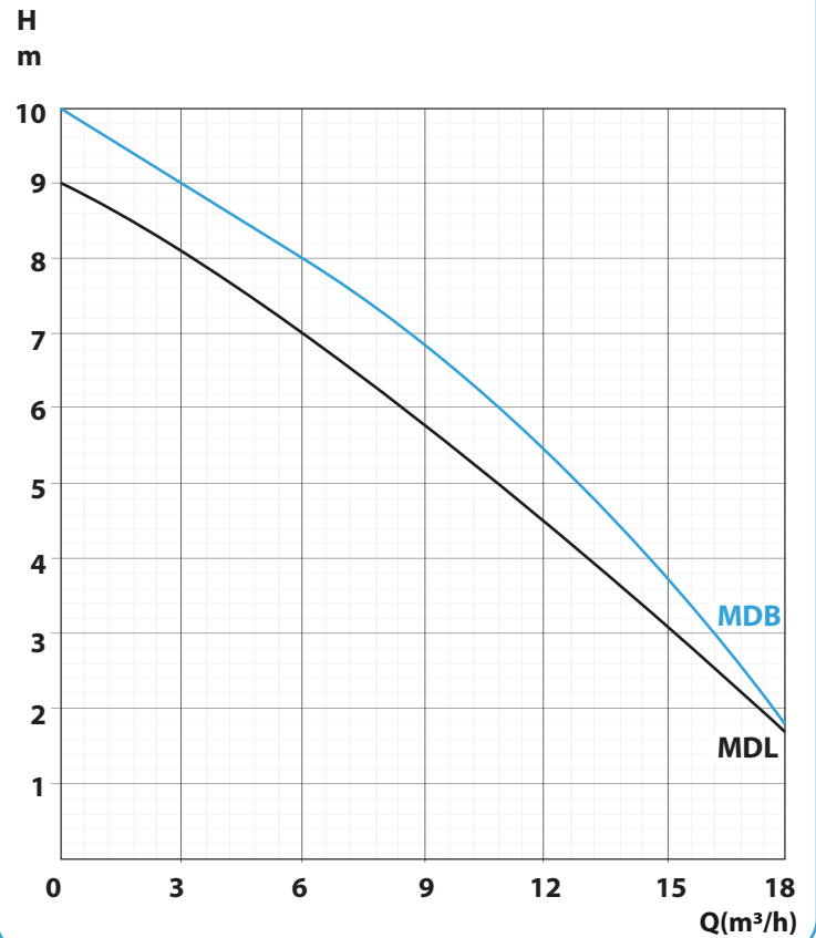
MDB & MDL Pump Performance Curve
