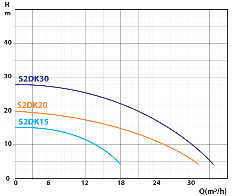
S2DK Pump Performance Curve
